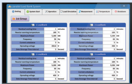
Loadbank controller
